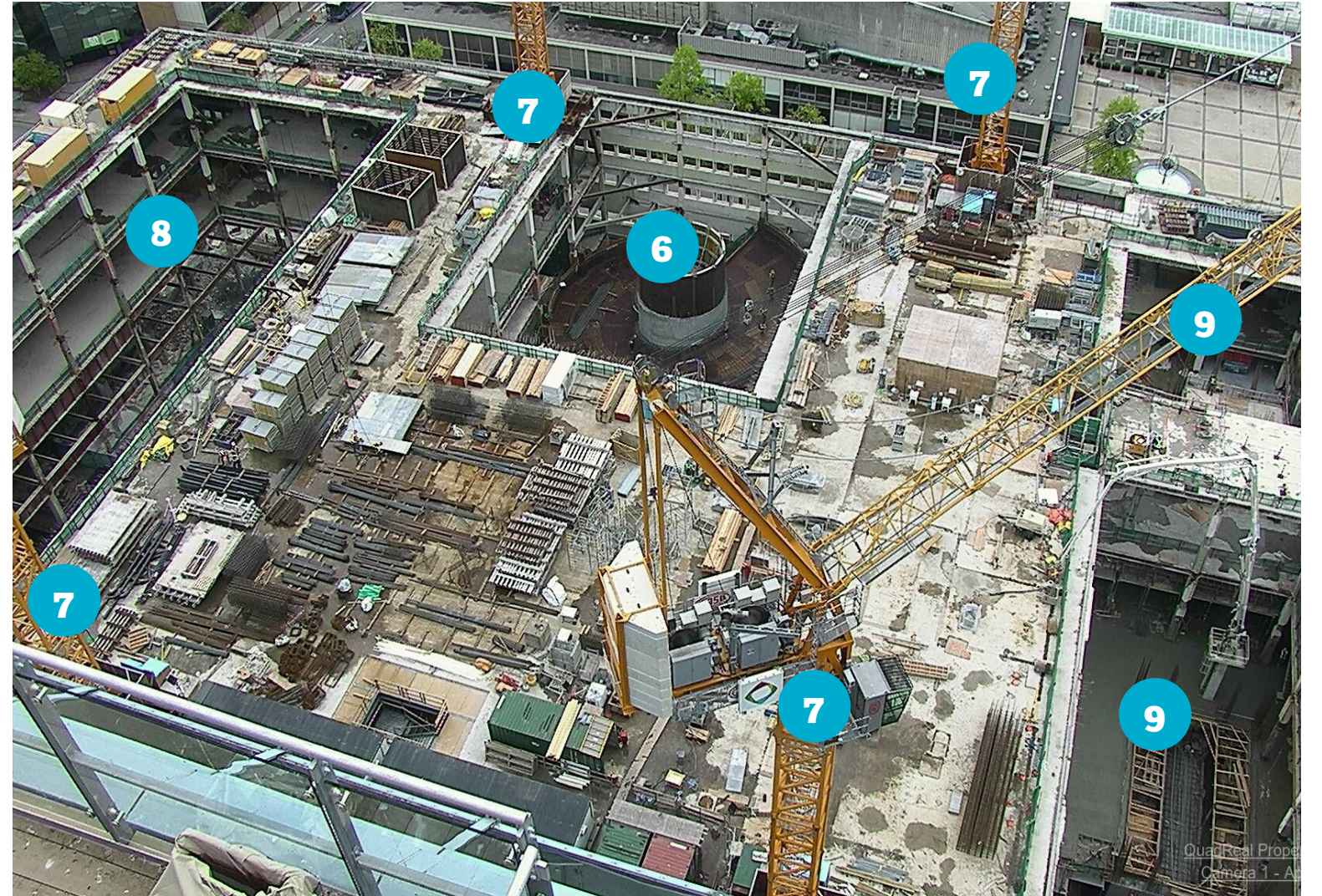
6 Opening in building for circular vehicle ramp
