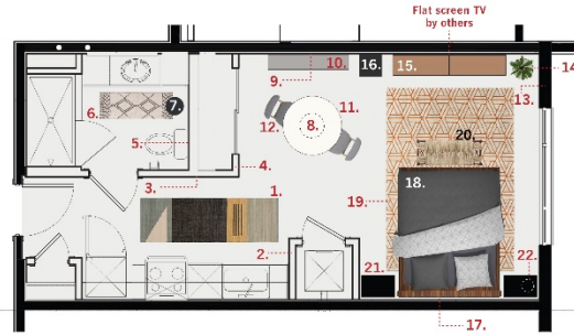
MODEL UNIT #303 FLOOR PLAN SCALE: 1/4" = 1'-0"
