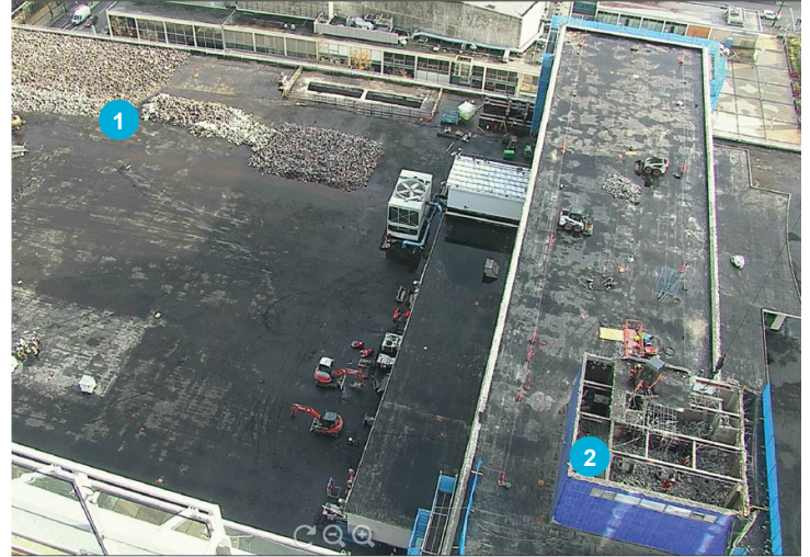
1 Asphalt and concrete topping being removed
